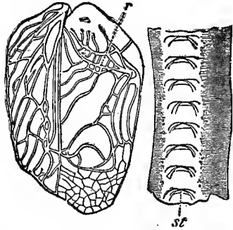
FIG. 11.— Gryllus campestris (from Landois). Right-hand figure, under side of part of a wing nerve, much magnified, showing the teeth, st . Left-hand figure, upper surface of wing-cover, with the projecting, smooth nervure, r , across which the teeth ( st ) are scraped.
